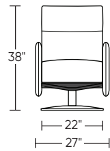
LUA-CHR-ST
